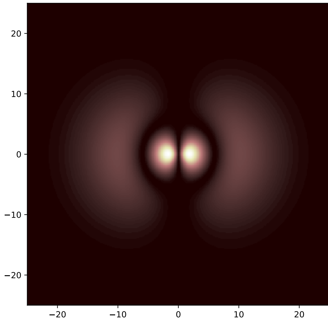
\rho(r, \theta, \phi = \text{whatever})
