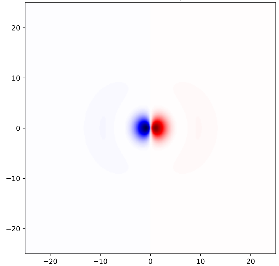
Probability current j_\phi(r, \theta)
